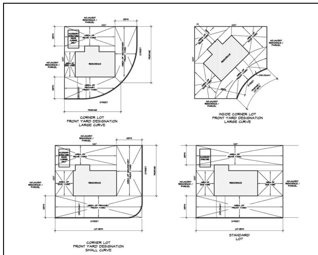
Figure 1. Front and Rear Yard Impervious Dimensional Criteria
